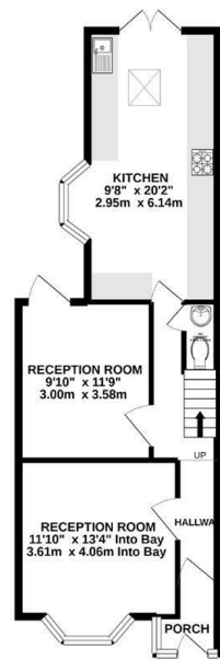
GROUND FLOOR 568 sq.ft. (52.8 sq.m.) approx.
