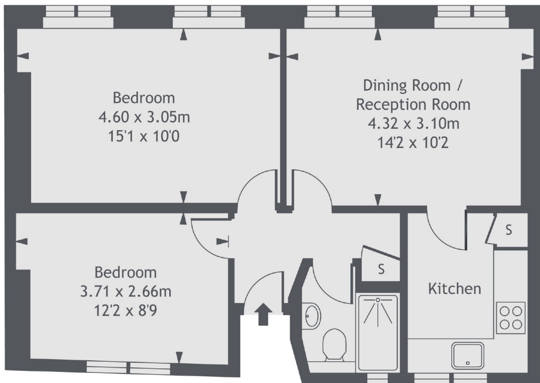
Third floor
