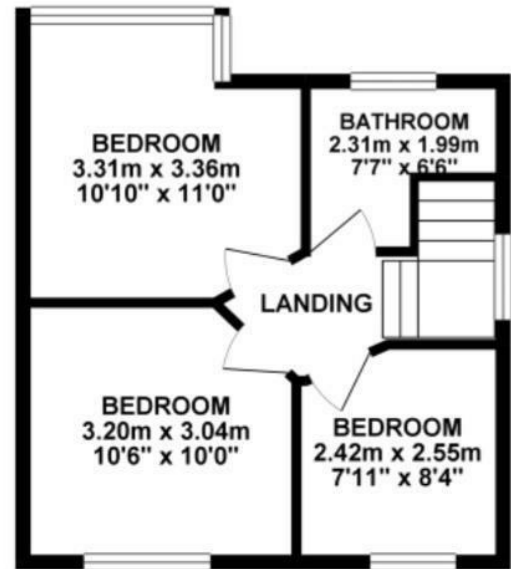
1ST FLOOR 33.40 sq. m. ( 359.46 sq. ft. )
