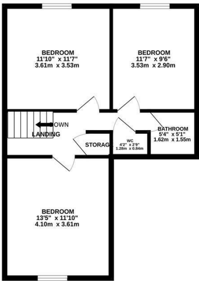
1ST FLOOR 515 sq.ft. (47.8 sq.m.) approx.
