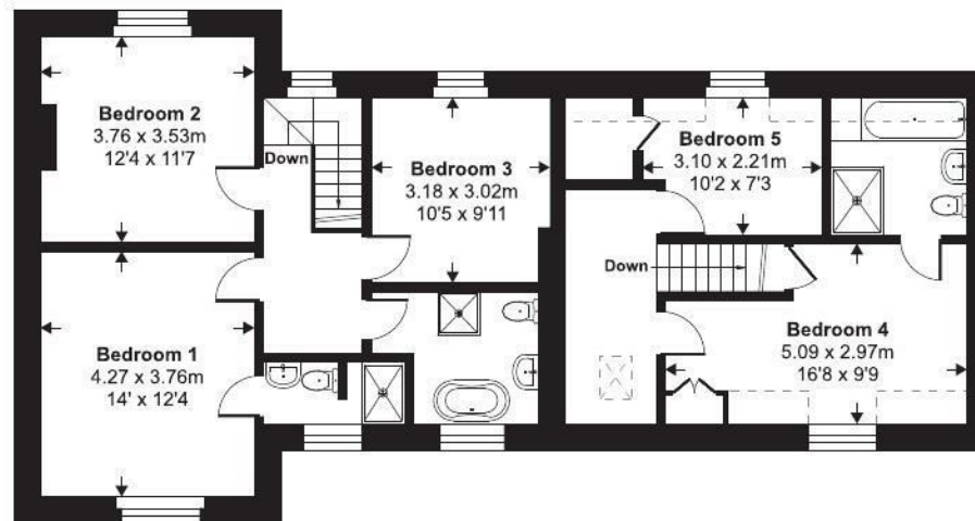
First Floor
