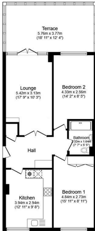
Floor Plan
