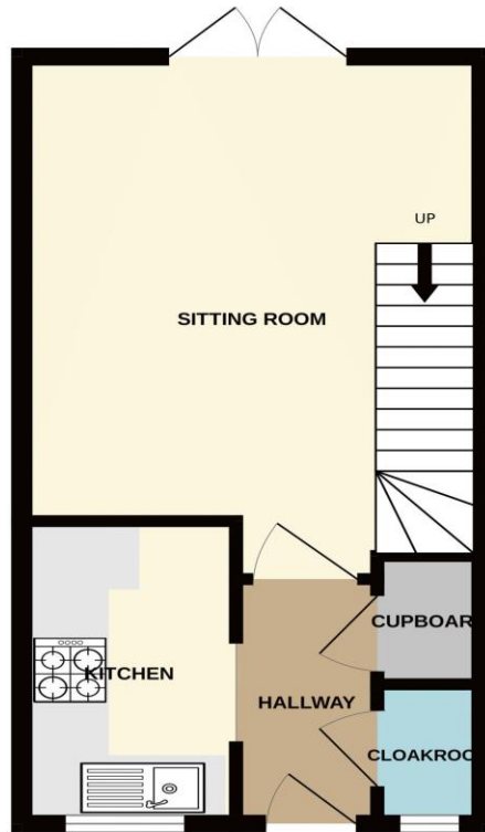
GROUND FLOOR 324 sq.ft. (30.1 sq.m.) approx.
