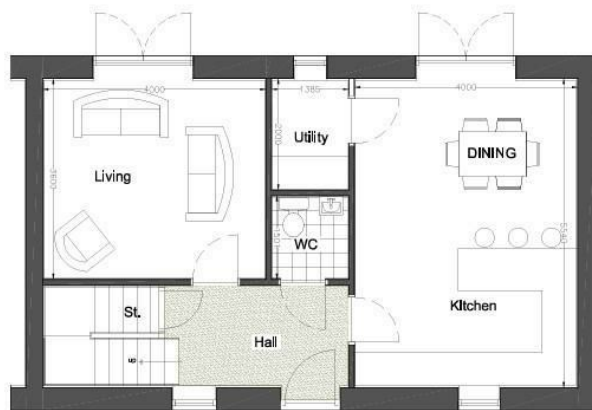
Plot 3 Ground Floor Plan
