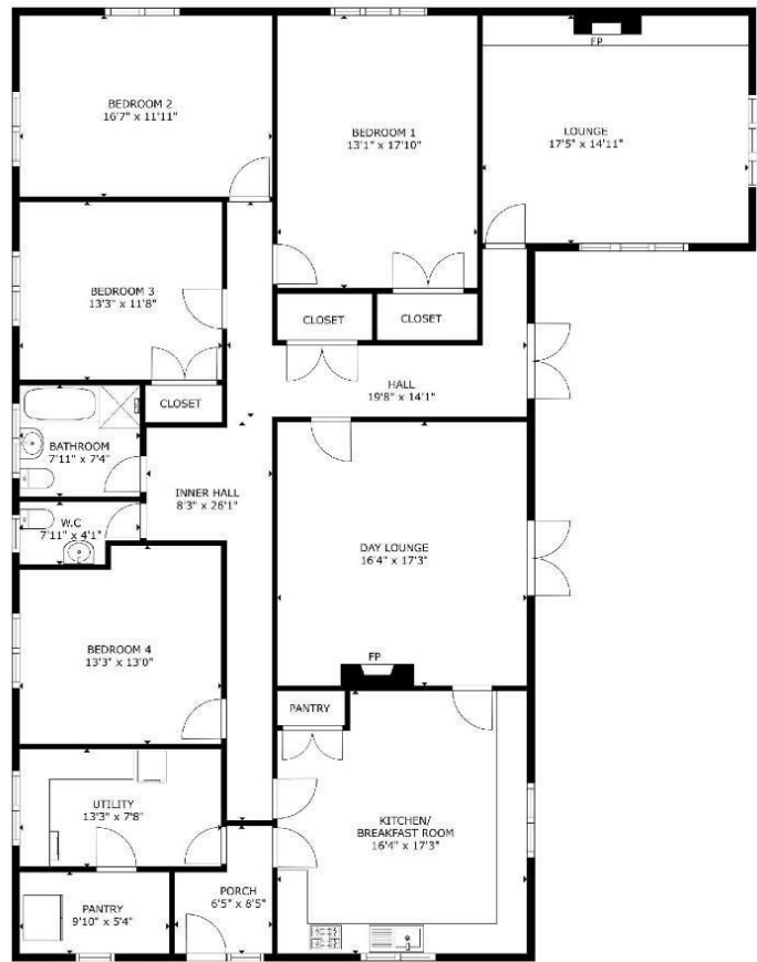
FLOOR PLAN
