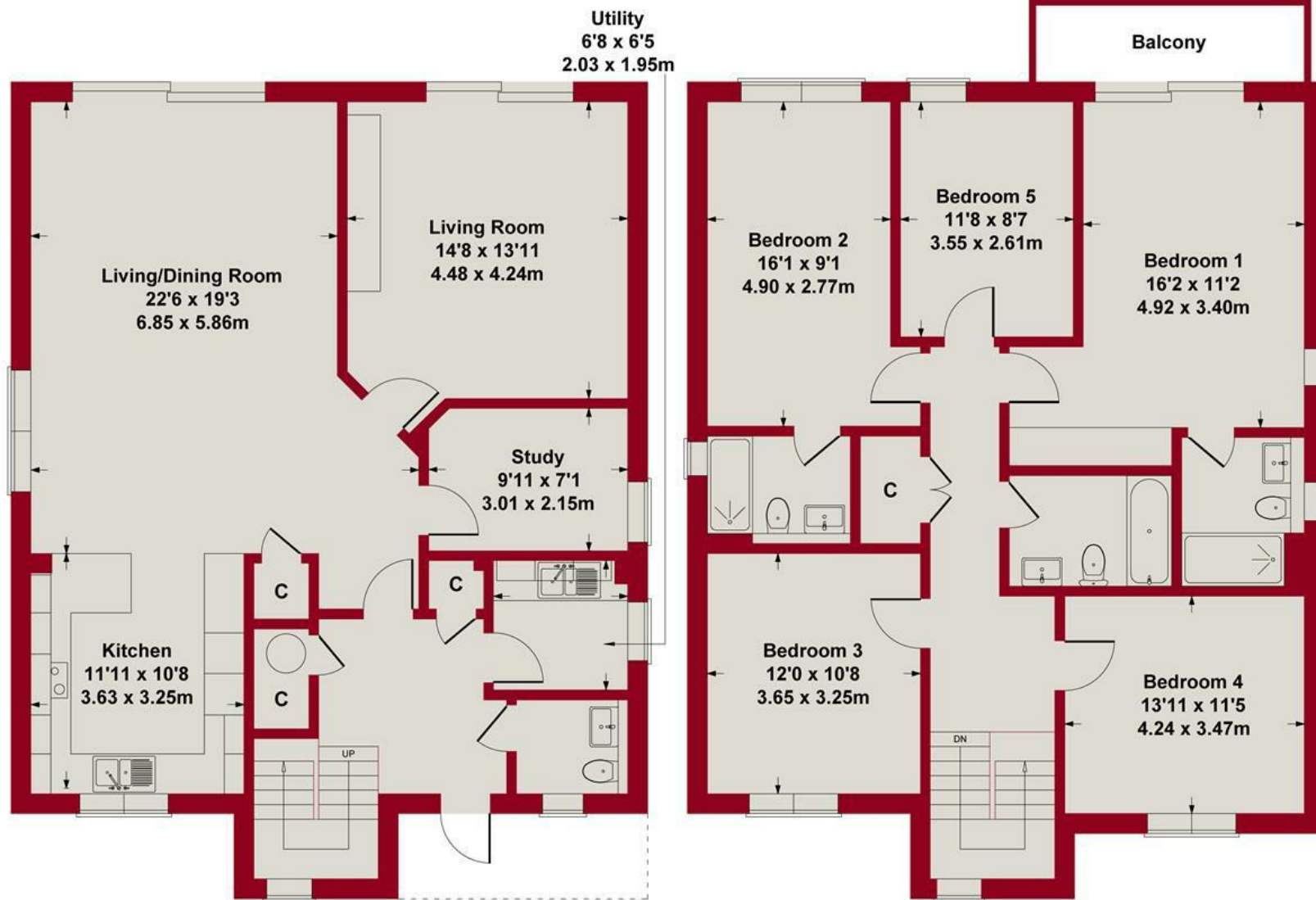
GROUND FLOOR
