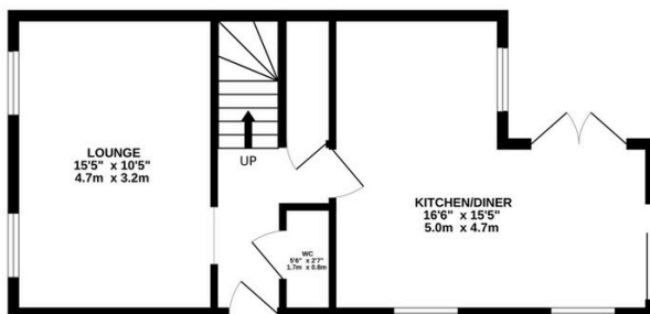
GROUND FLOOR 458 sq.ft. (42.5 sq.m.) approx.
