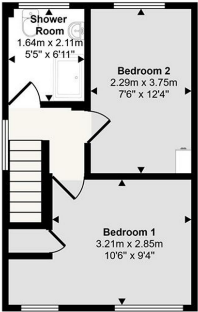
First Floor Approx 28 sq m / 298 sq ft
