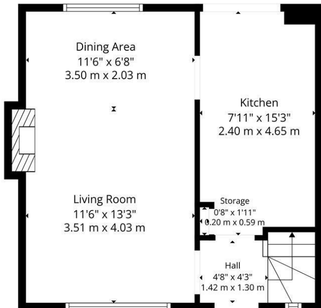
1st Floor
