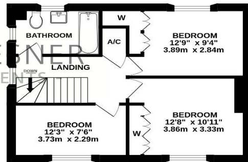
1ST FLOOR 479 sq.ft. (44.5 sq.m.) approx.
