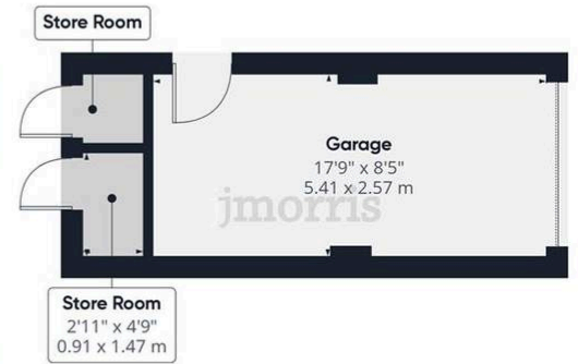
Ground Floor Building 2
