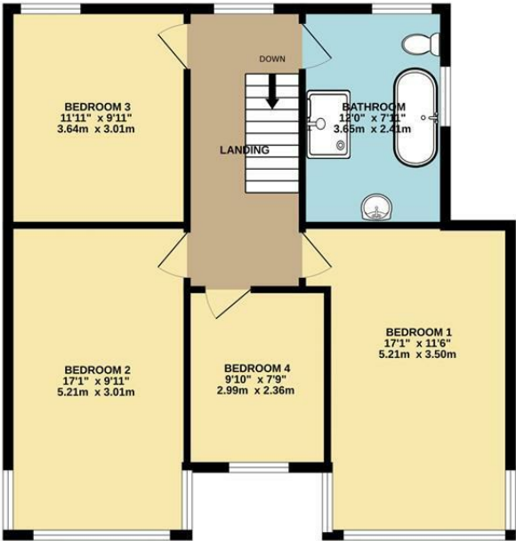
1ST FLOOR 734 sq.ft. (68.2 sq.m.) approx.
