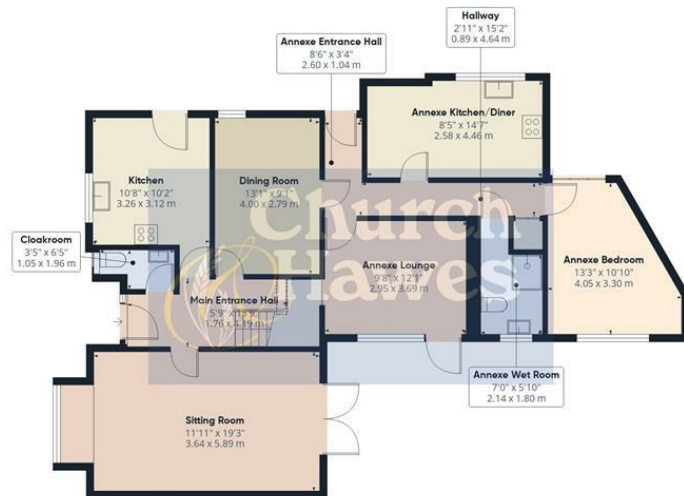
Floor 0 Building 1
