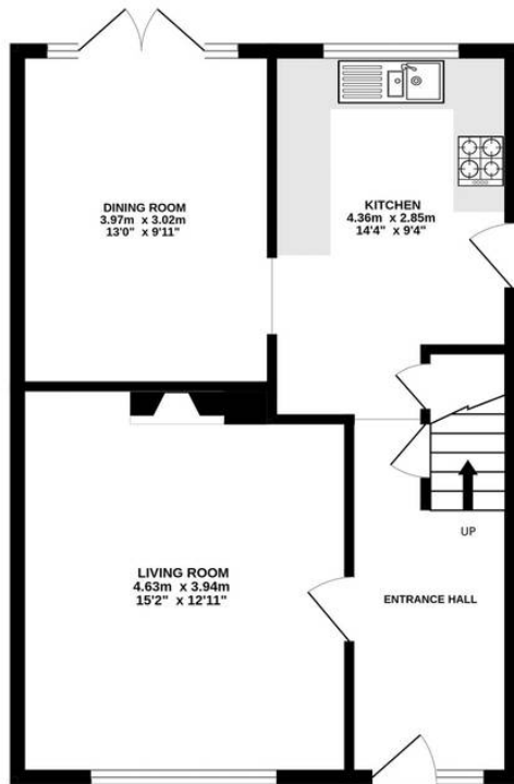
GROUND FLOOR 63.8 sq.m. (687 sq.ft.) approx.
