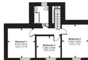
Farmhouse First Floor
