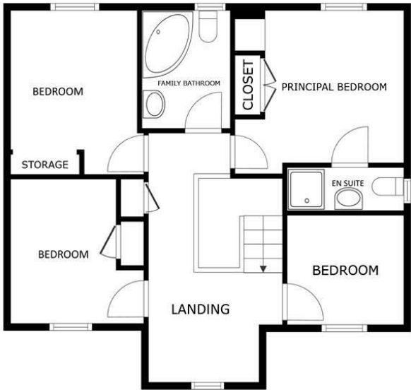
FLOOR 2
