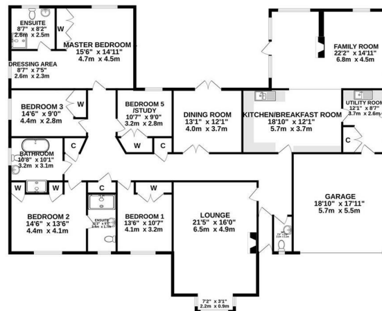
GROUND FLOOR 3023 sq.ft. (280.8 sq.m.) approx.
