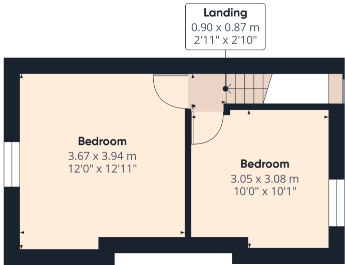
Floor 1 Building 1
