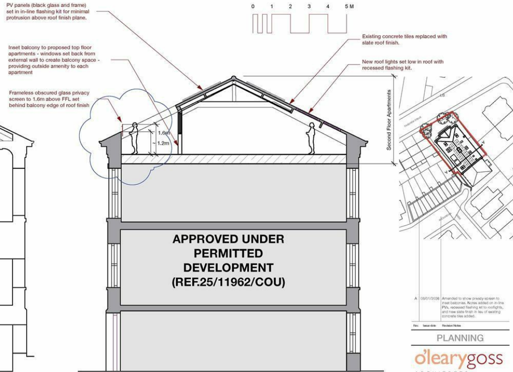
Proposed Section
