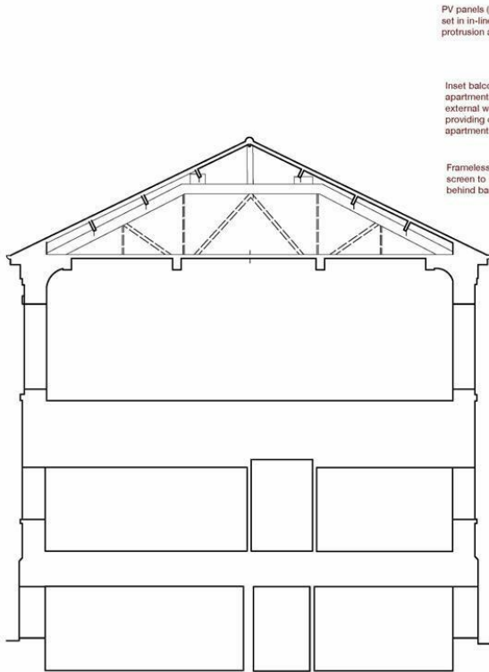
Existing Section
