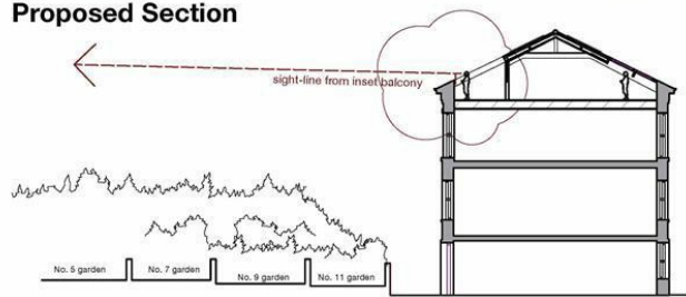
Overlooking Section
