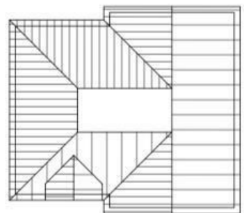
Proposed Roof Plan Scale 1:50
