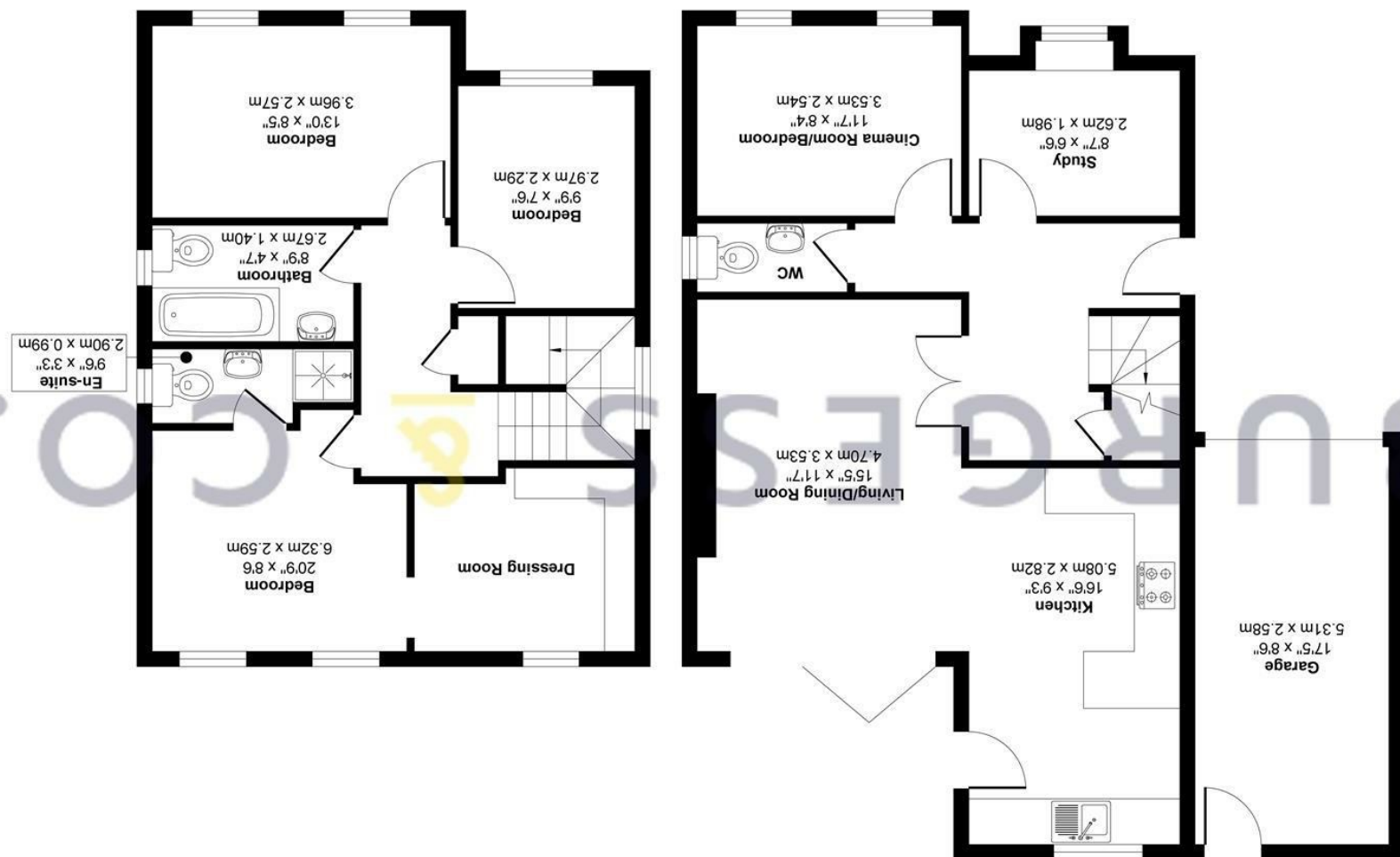
GROUND FLOOR
