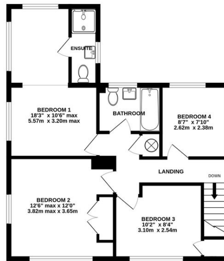
1ST FLOOR 629 sq.ft. (57.9 sq.m.) approx.
