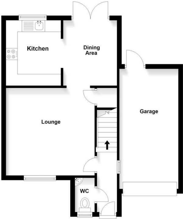
Ground Floor Approx. 49.5 sq. metres (532.9 sq. feet)
