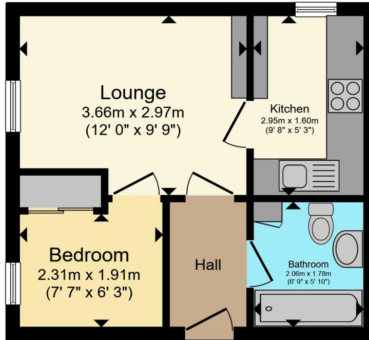
Floor Plan
