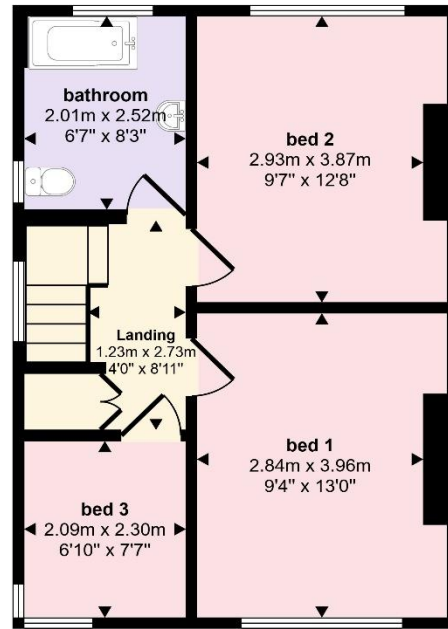
First Floor Approx 43 sq m / 459 sq ft
