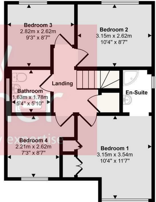
First Floor Approx 47 sq m / 506 sq ft
