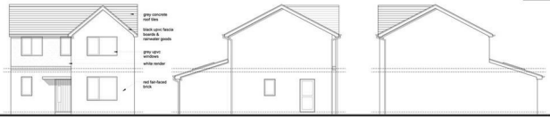
FRONT ELEVATION (EAST)
