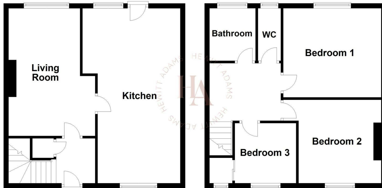
Ground Floor
