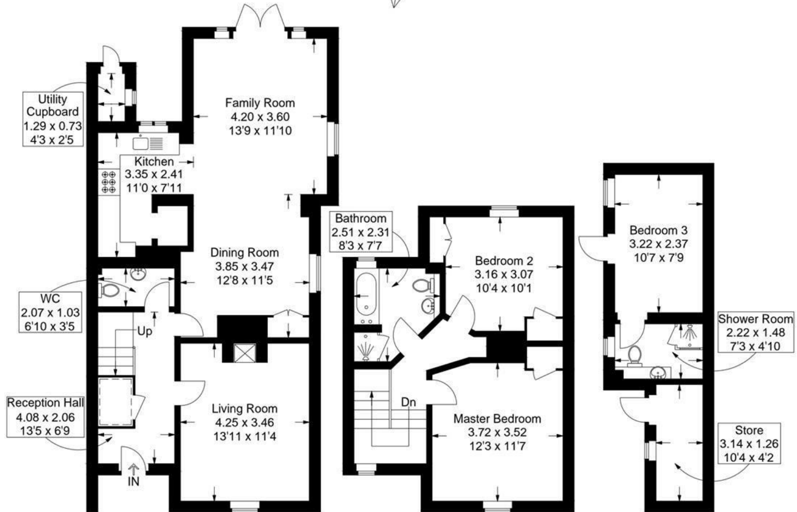
Ground Floor
