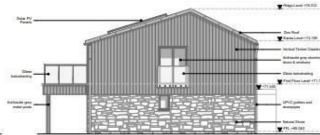
PROPOSED NORTH ELEVATION 1:100
