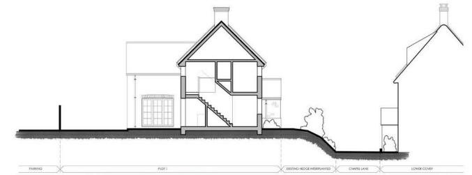
SITE SECTION AA proposed - scale 1:200
