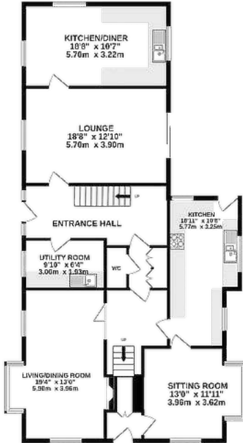
GROUND FLOOR 1286 sq.ft. (119.4 sq.m.) approx.
