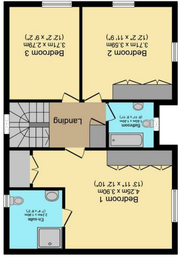
First Floor Floor area 60.4 m 2 (650 sq.ft.)
