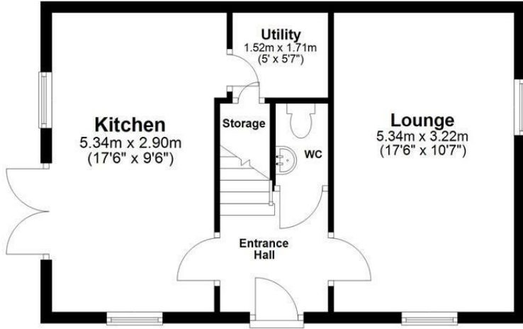
Ground Floor Approx. 42.9 sq. metres (461.4 sq. feet)
