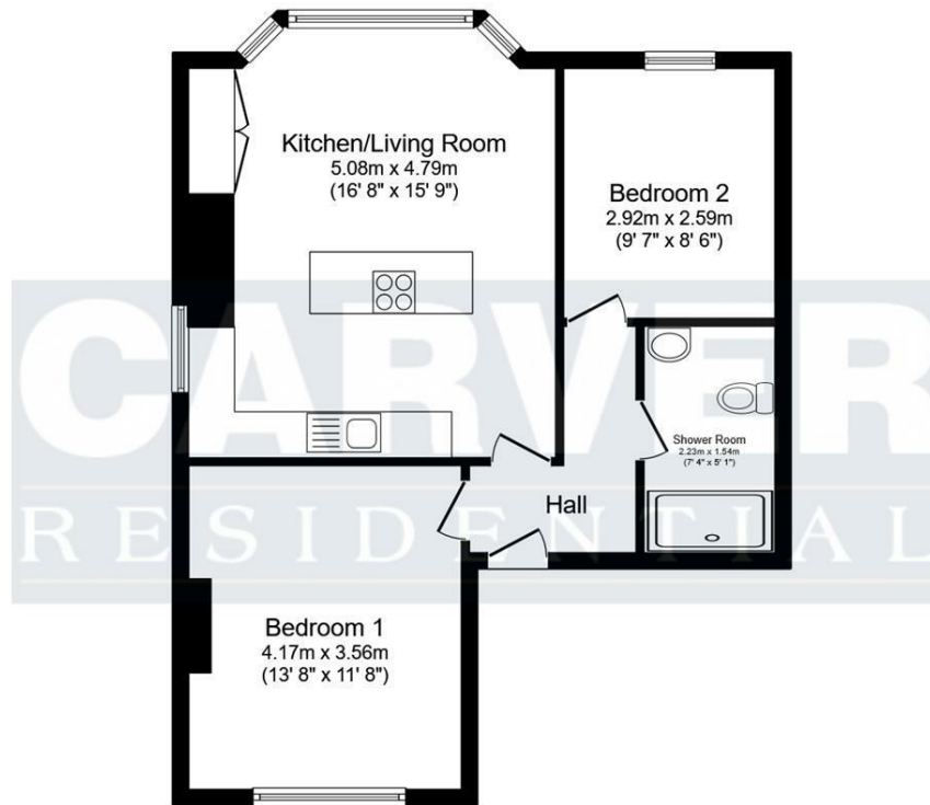
First Floor Floor area 61.0 sq.m. (657 sq.ft.)
