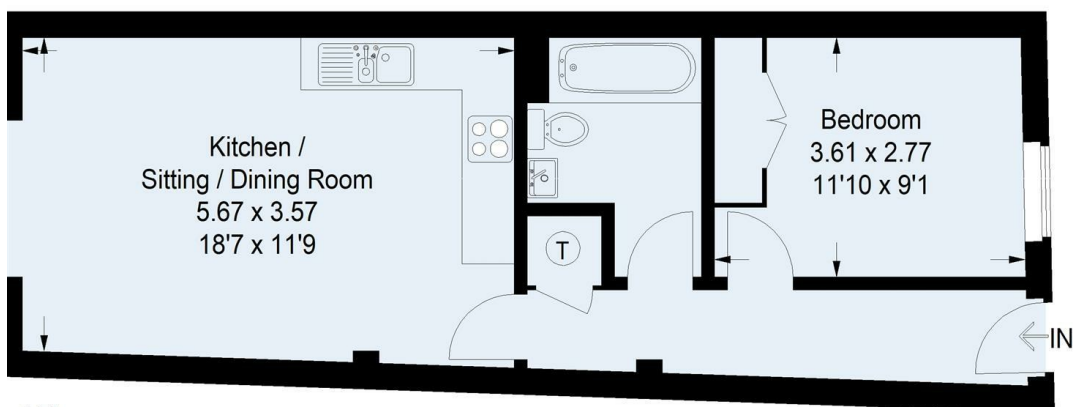
1st Floor
