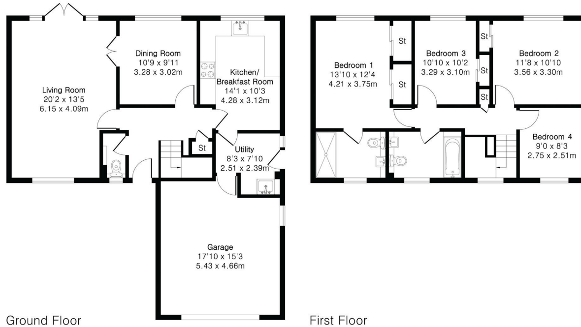
Ground Floor
