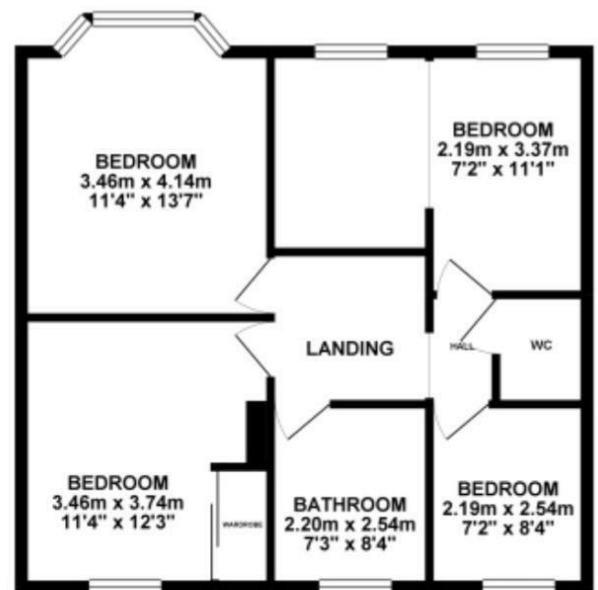
1ST FLOOR 59.10 sq. m. ( 636.20 sq. ft. )
