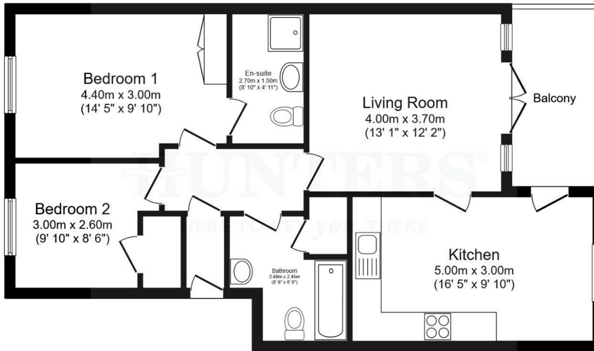
Floor Plan Floor area 68.7 sq.m. (740 sq.ft.)
