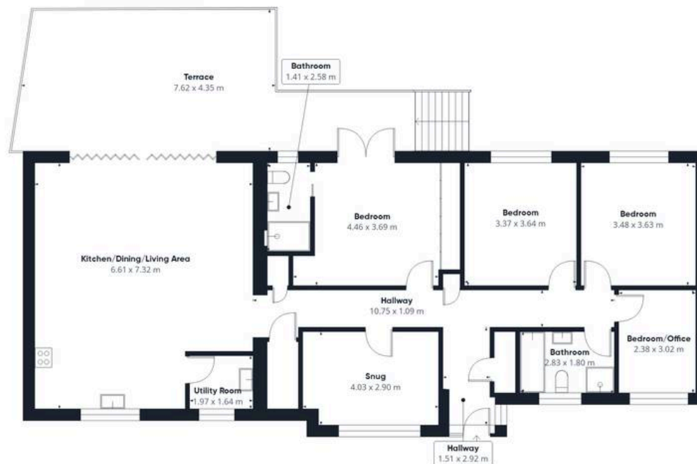
Floor 0 Building 1
