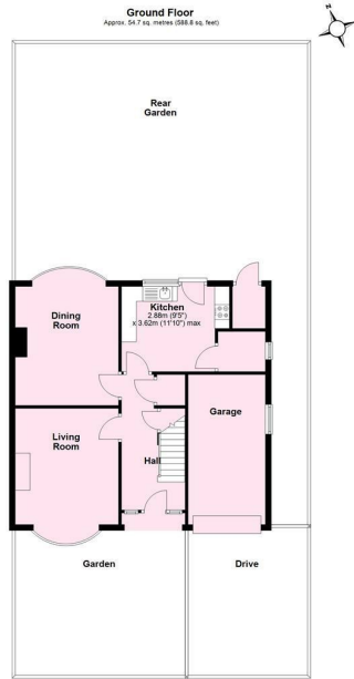
Total area: approx. 54.7 sq. metres (588.8 sq. feet) Not to scale for illustrative purposes only. Approximate gross internal floor area. (Excluding stairs and any storage). All measurements and figures including doors and windows are approximate and should be independently verified. Plan produced using PlanIt.
