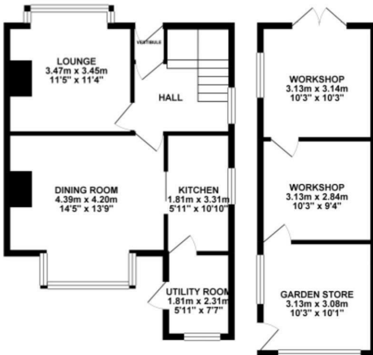
GROUND FLOOR 74.81 sq. m. ( 805.26 sq. ft. )
