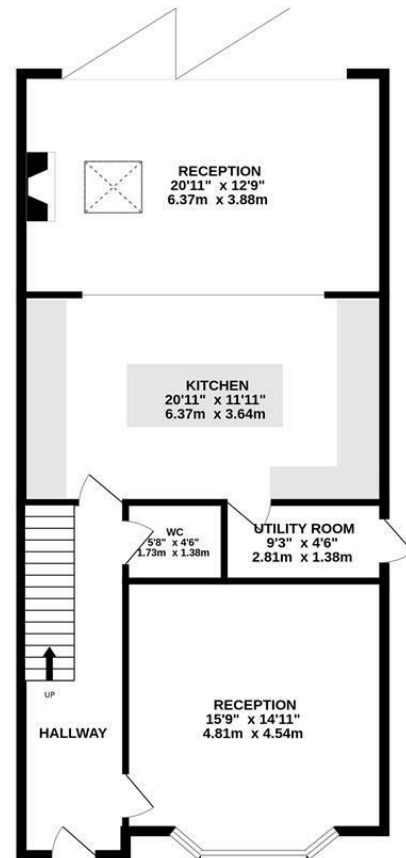
GROUND FLOOR 924 sq.ft. (85.8 sq.m.) approx.
