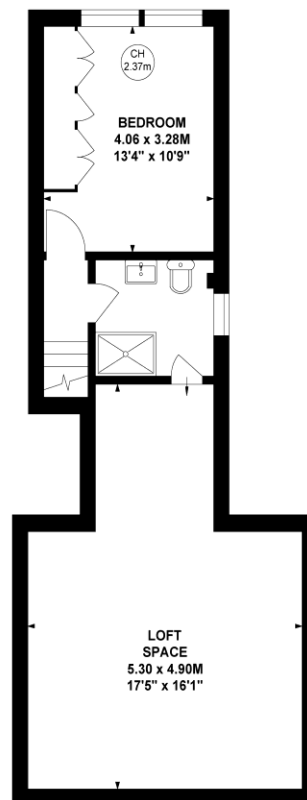
Second Floor
