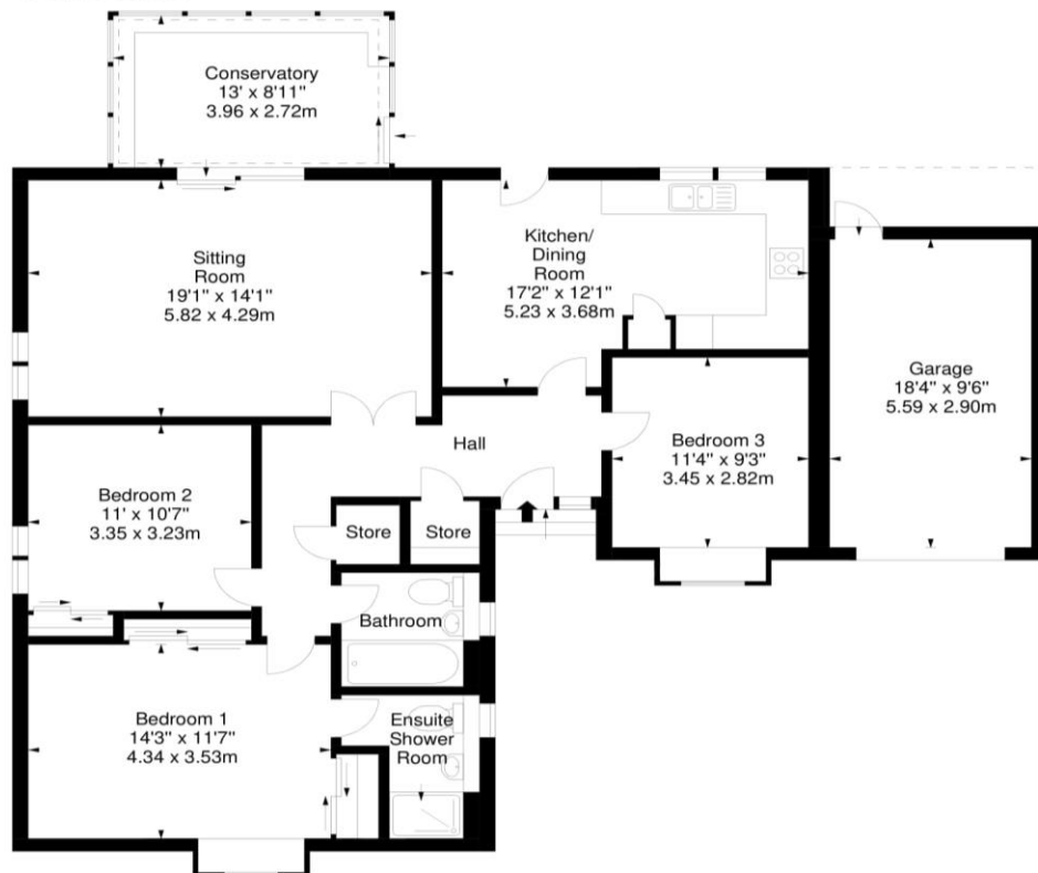
Ground Floor
