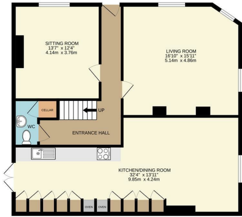
GROUND FLOOR 946 sq.ft. (87.8 sq.m.) approx.
